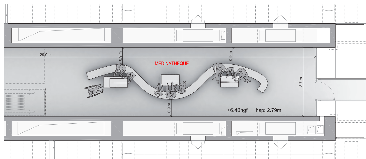
MEDINATHEQUE - PLAN 1/100
